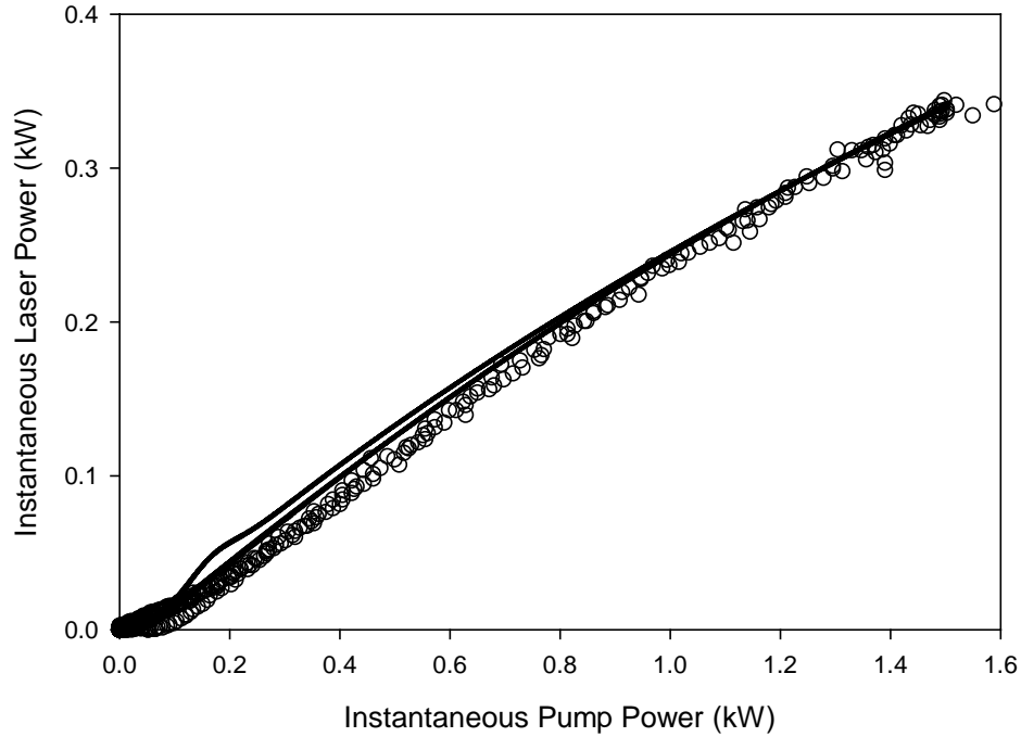
Figure 29. Instantaneous laser power vs. pump power for the model (-) and data (○), with a 5 ns delay of the pump pulse.
