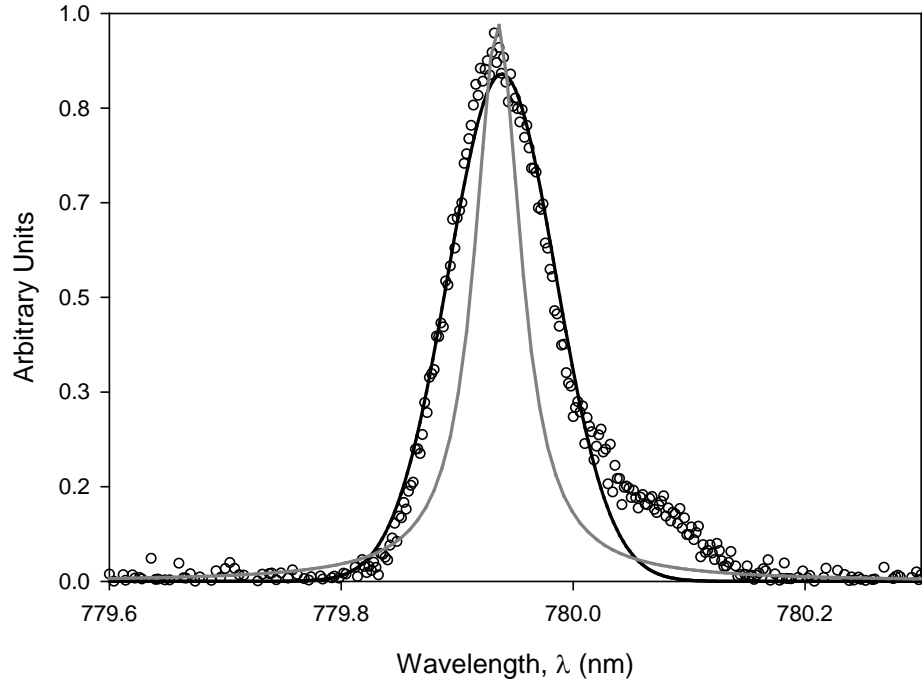
Figure 23. Bandwidth of (○) Ti:Sapphire pump when DML-100 green pump source was used with ~ 42 GHz wide (-) Gaussian and a (-) Lorentzian with a typical pressure broadened absorption line.
