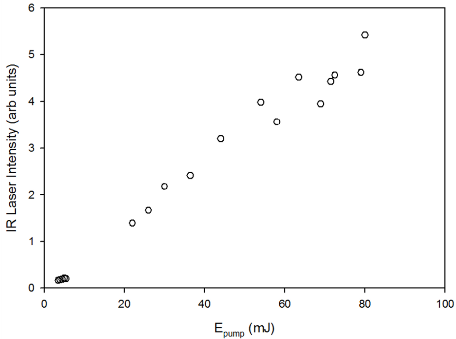
Figure 46. Infrared beam energy after pulsed laser pumping of the Cs 6^2S_{1/2} - 7^2D_{3/2} transition at a cell temperature of (o) 185 °C.
