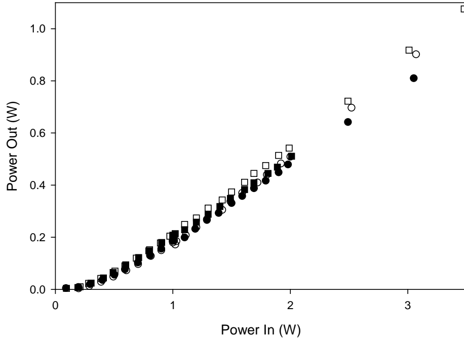
Figure 32. Output vs input power at T=120\text{C} and R_{oc}=20\% . Buffer gases of ( \circ )300 Torr \text{C}_2\text{H}_6 / 200 Torr He, ( \square )450 Torr \text{C}_2\text{H}_6 / 200 Torr He, ( \bullet )450 Torr \text{C}_2\text{H}_6 , and ( \square )600 Torr \text{C}_2\text{H}_6 are shown.
