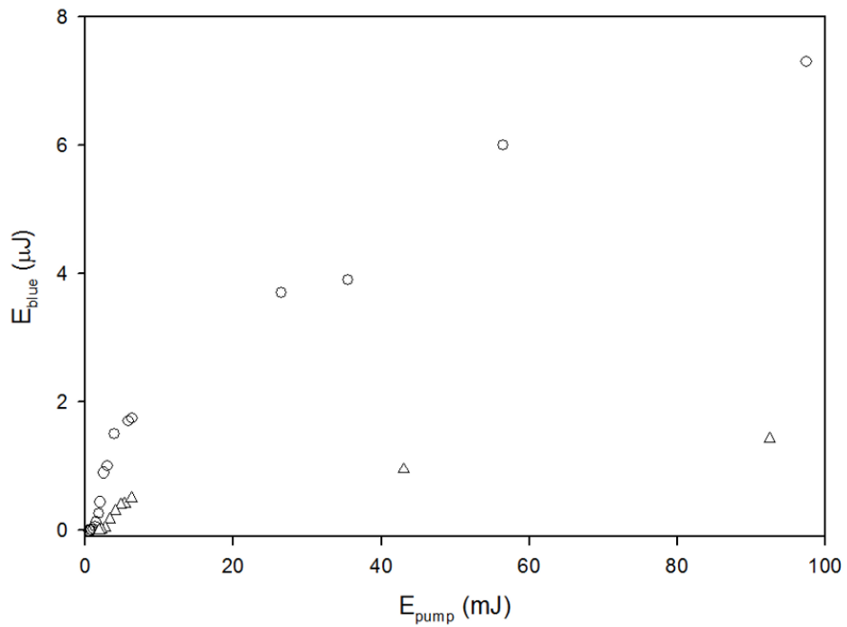
Figure 45. Blue 6^2P_{3/2,1/2} - 5^2S_{1/2} beam energy after pulsed laser pumping of the Cs 6^2S_{1/2} - 7^2D_{3/2} transition at cell temperatures of: ( \Delta ) 175 °C and (o) 200 °C.
