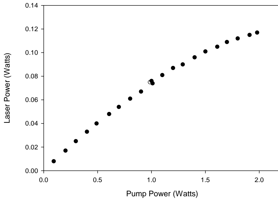
Figure 58. P_{ethane} = 450 Torr, R_{OC} = 50\% , T = 80^{\circ}\text{C}
