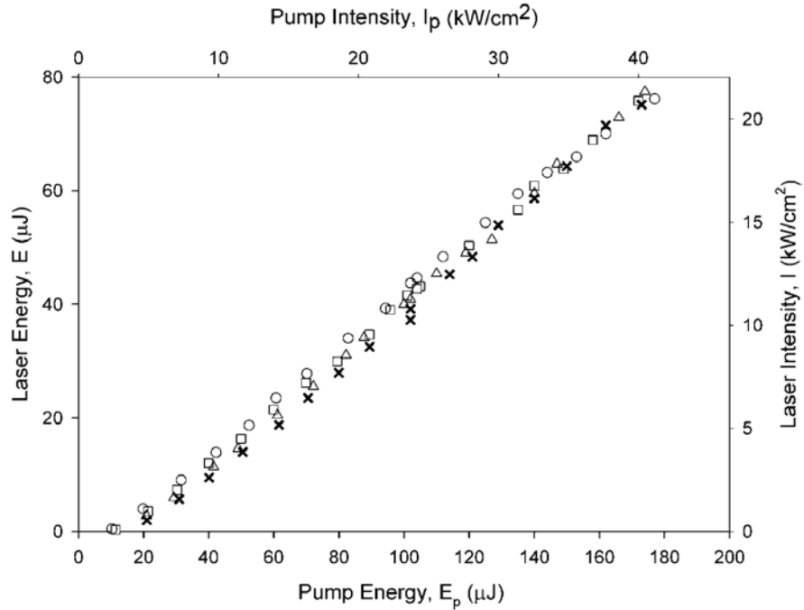
Figure 16. Rb laser output energy per pulse as a function of input laser energy for the 32% output coupler and cell temperatures of (X) 393 K, (□) 390 K, (◻) 387 K, and (○) 382 K.
