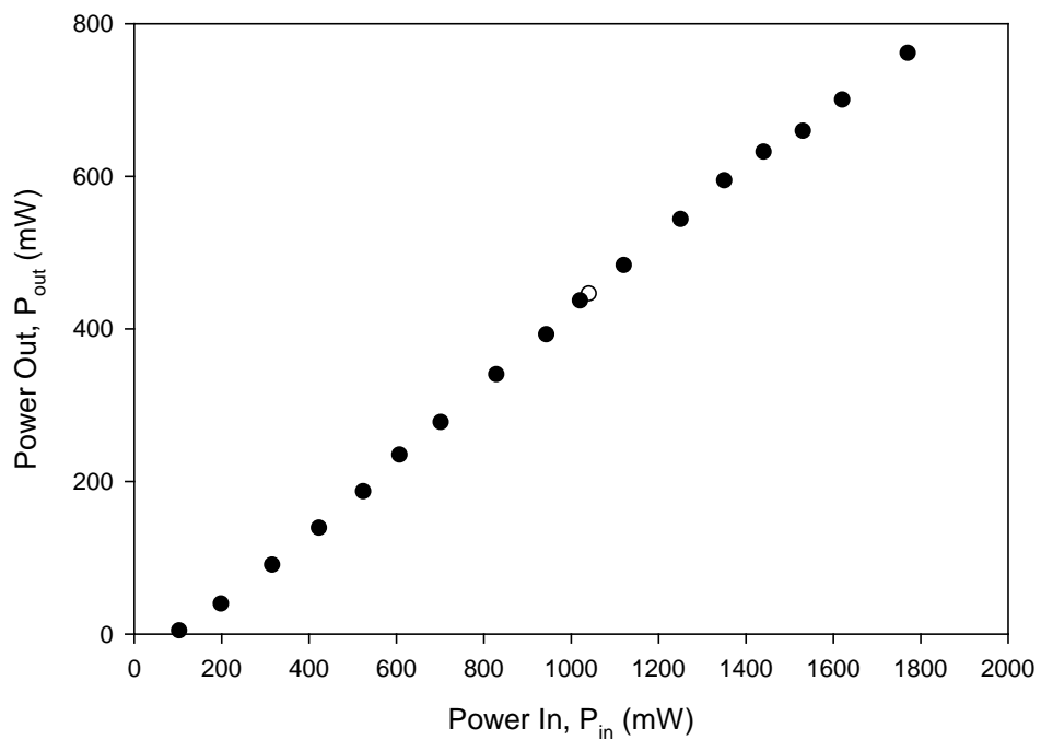
Figure 50. P_{methane} = 550 Torr, R_{OC} = 32\% , T = 109^{\circ}\text{C}
