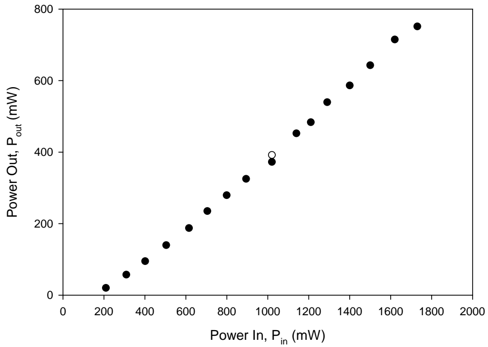
Figure 53. P_{methane} = 550 Torr, R_{OC} = 32\% , T = 120^{\circ}\text{C}
