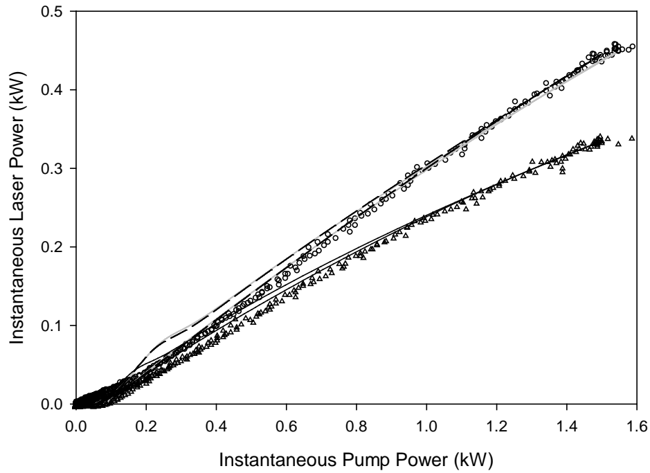
Figure 34. Instantaneous slope efficiency data compared to model with T=100\text{C} and R_{oc}=20\% . Collected data with buffer gases of (○) 300 Torr \text{C}_2\text{H}_6 / 200 Torr He, and (□) 450 Torr \text{C}_2\text{H}_6 are shown, as well as model results for (□) 300 Torr \text{C}_2\text{H}_6 / 200 Torr He, and (--) 450 Torr \text{C}_2\text{H}_6 , additionally model results for (□) 450 Torr \text{C}_2\text{H}_6 incorporating a 62.5% decrease in concentrations of alkali number density and spin orbit gas.
