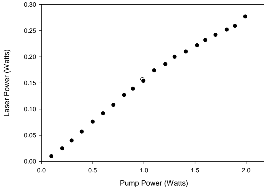
Figure 57. P_{ethane} = 450 Torr, R_{OC} = 50\% , T = 90^{\circ}\text{C}
