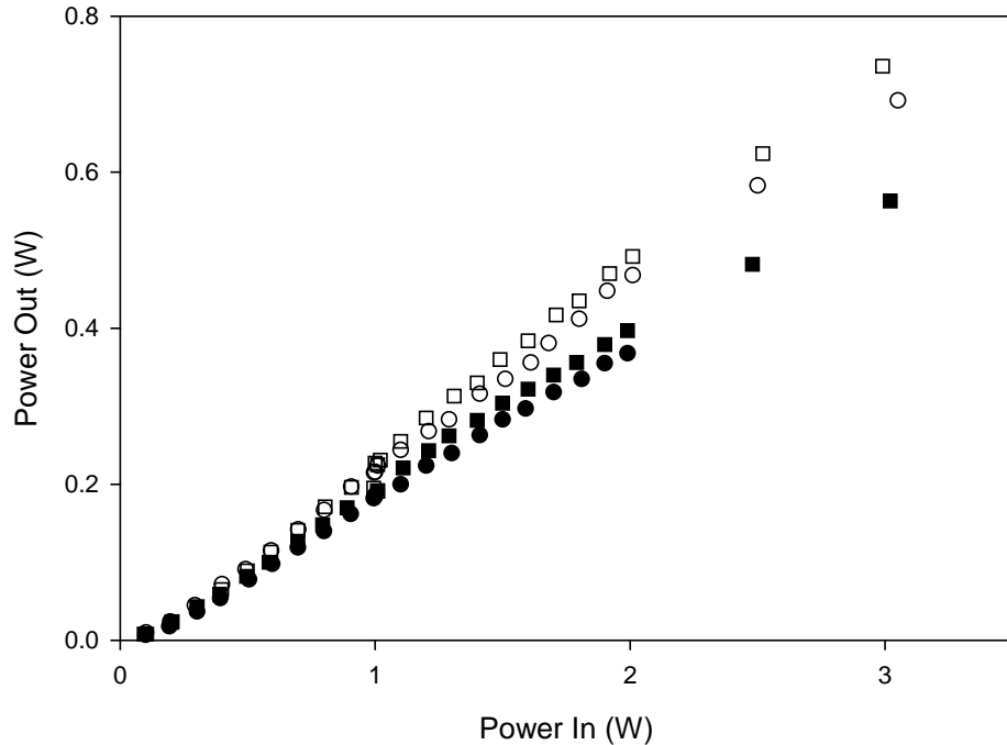
Figure 33. Dependence of output power on input power at T=100\text{C} and R_{oc}=20\% . Buffer gases of ( \circ ) 300 Torr \text{C}_2\text{H}_6 / 200 Torr He, ( \square ) 450 Torr \text{C}_2\text{H}_6 / 200 Torr He, ( \bullet ) 450 Torr \text{C}_2\text{H}_6 , and ( \square ) 600 Torr \text{C}_2\text{H}_6 are shown.
