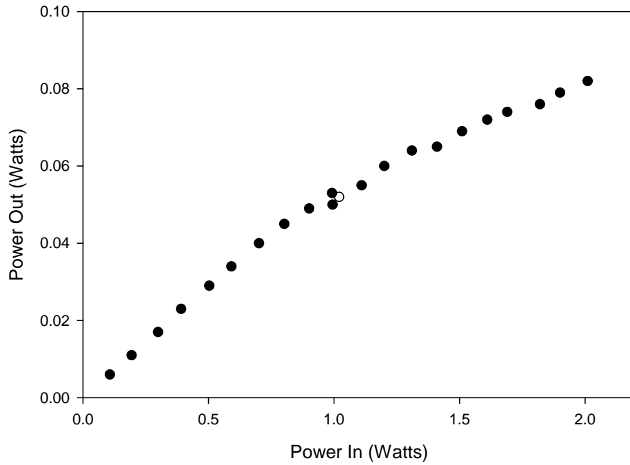
Figure 66. P_{ethane} = 450 Torr, R_{OC} = 70\% , T = 80^{\circ}\text{C}
