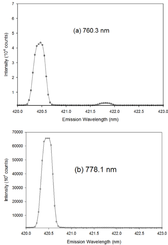
Figure 41. Spectrally resolved blue beam intensity from the Rb cell, when pumped on the: (a) 5^2S_{1/2} - 7^2S_{1/2} line at 760.3 nm, and the (b) 5^2S_{1/2} - 5^2D_{3/2} line at 778.1 nm.
